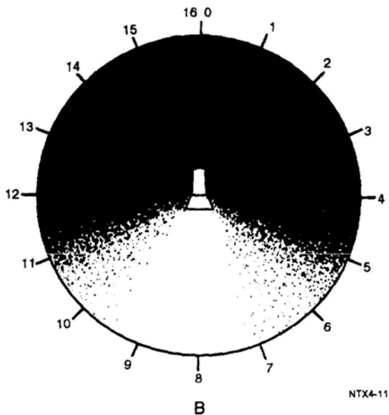
Figure 2-6.—Anisotropic radiator.
