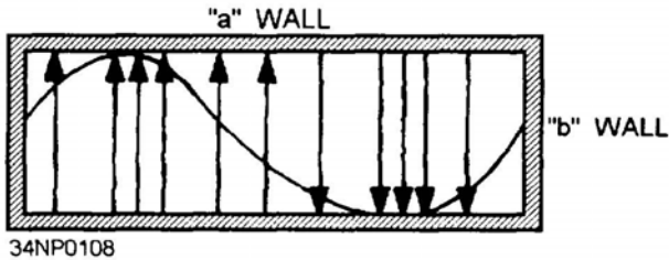
Figure 3-35.—Full-sine E field distribution.
