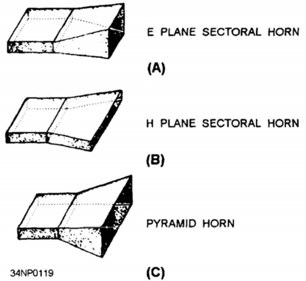
Figure 3-46.—Waveguide horns.
