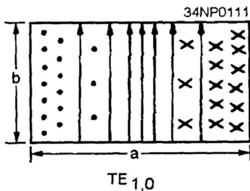
Figure 3-38.—TE 1,0 mode in a rectangular waveguide.
