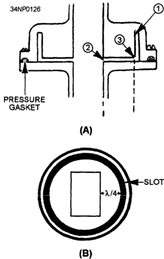
Figure 3-53.—Choke joint.
