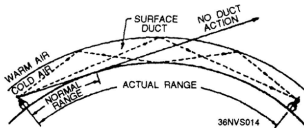
Figure 1-14.—Duct effect caused by temperature inversion.
