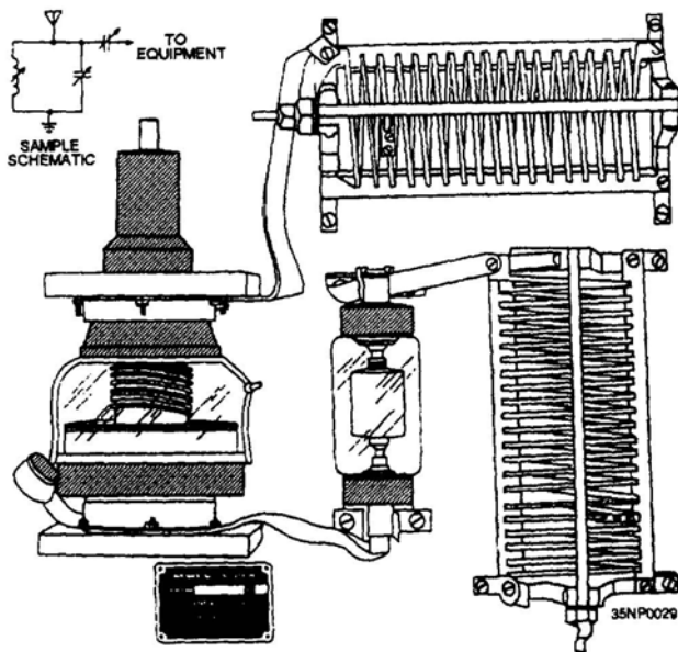
Figure 2-37.—Matching network.
