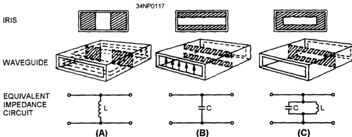
Figure 3-44.—Waveguide irises.
