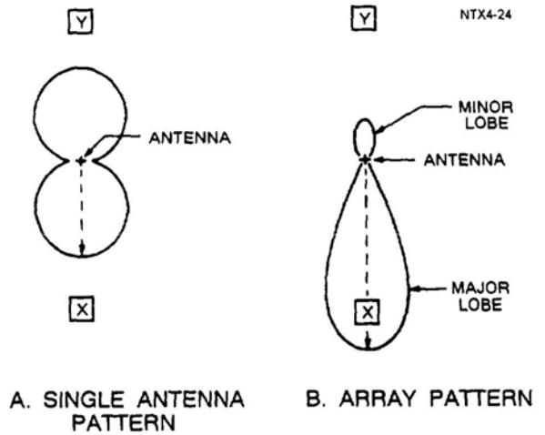
Figure 2-7.—Major and minor lobes.
