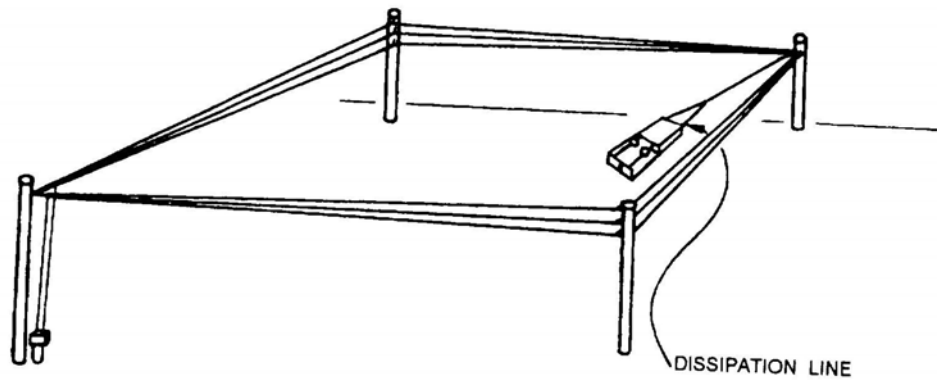
B. NON - RESONANT HORIZONTAL THREE - WIRE RHOMBIC
