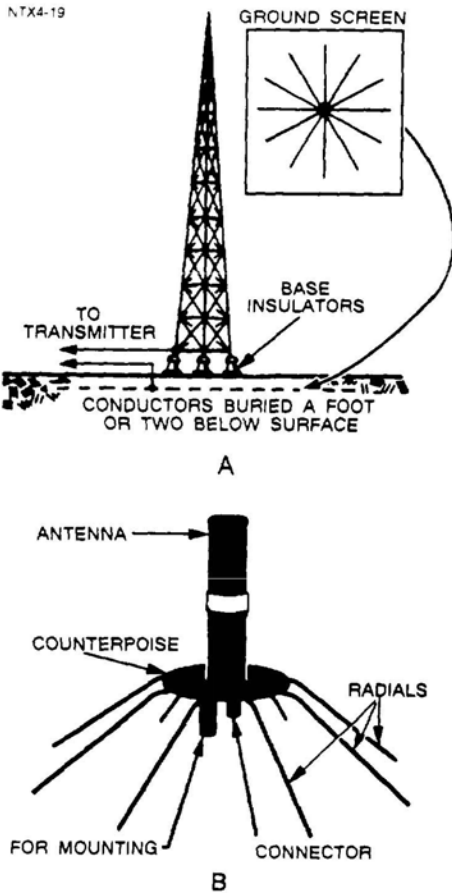
Figure 2-9.—Ground screen and counterpoise.
