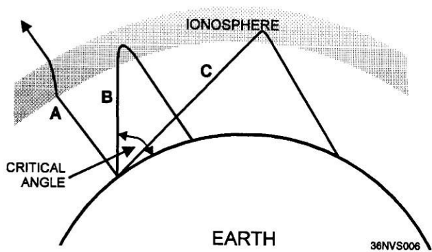
Figure 1-6.—Incidence angles of radio waves.
