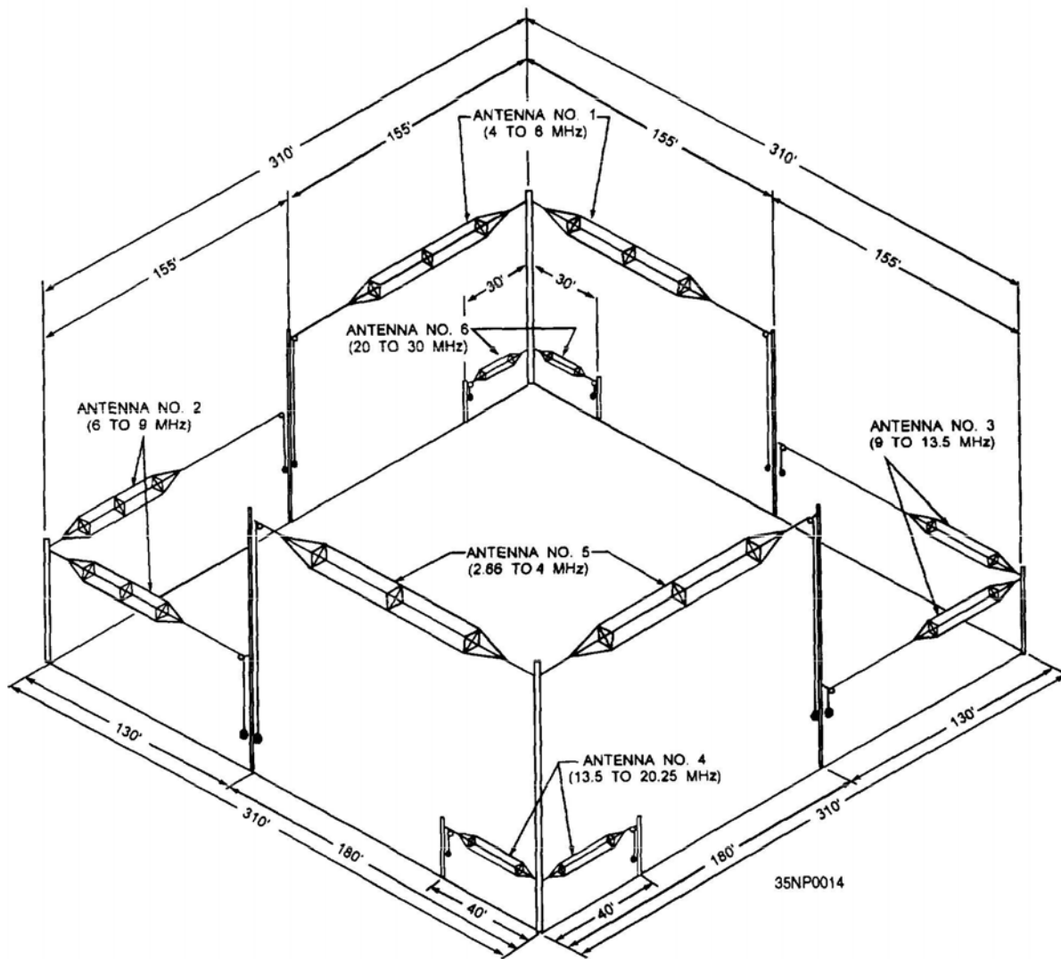
Figure 2-22.—Quadrant antenna.
