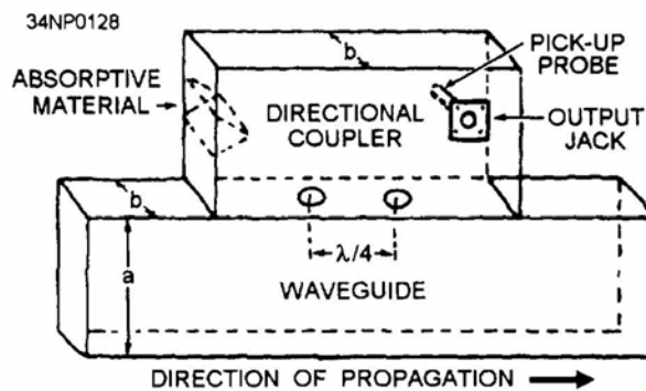
Figure 3-55.—Directional coupler.
