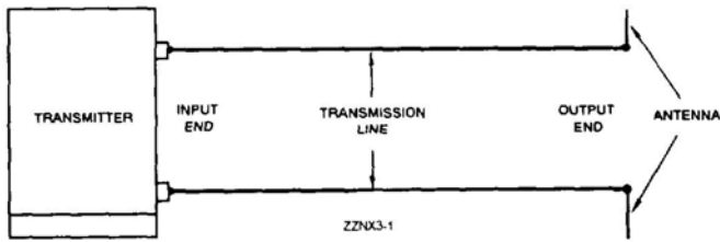
Figure 3-9.—Two-wire open line.
