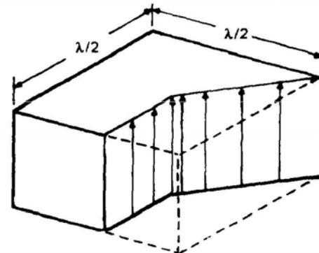
ELECTRIC FIELD PATTERN
