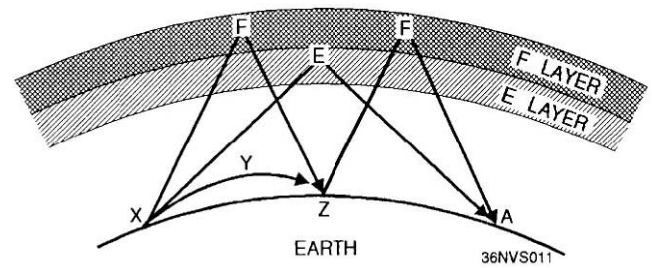
Figure 1-11.—Multipath transmission.
