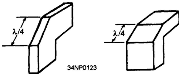
Figure 3-50.—Sharp bends.
